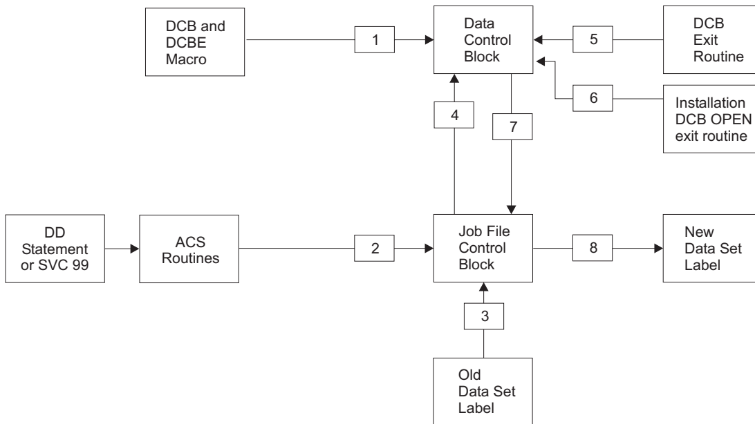
Figure 53. Sources and Sequence of Operations for Completing the DCB
