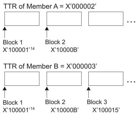
Figure 87. TTRs for Two PDSE Members (LRECL=80, BLKSIZE=800)
