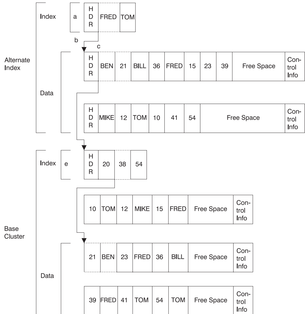
Figure 18. Alternate Index Structure for a Key-Sequenced Data Set
