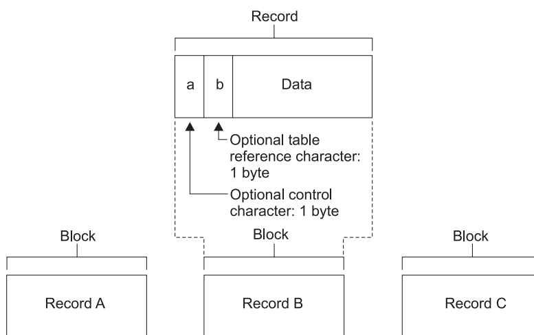
Figure 47. Undefined-Length Records
