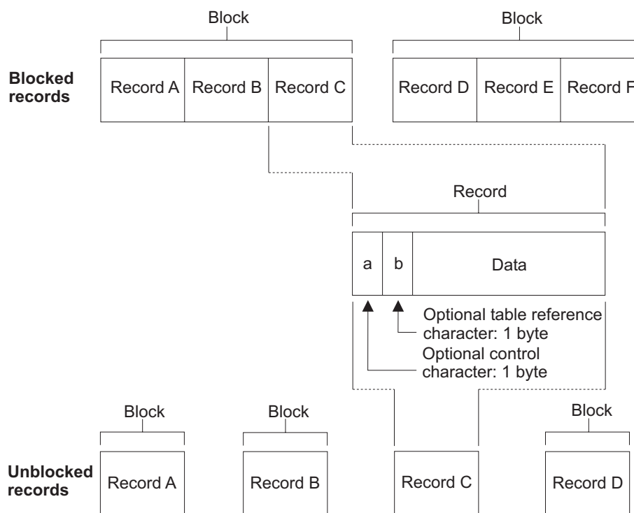
Figure 43. Fixed-Length Records
