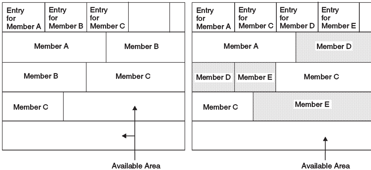
Figure 85. A Partitioned Data Set Extended (PDSE)
