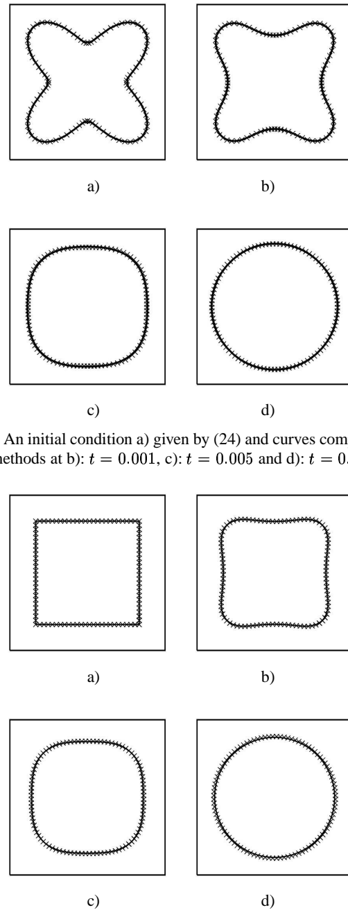
Fig. 4. A square as an initial condition a) and computed evolved curves b): t = 0.001 , c): t = 0.01 and d): t = 0.1 .
