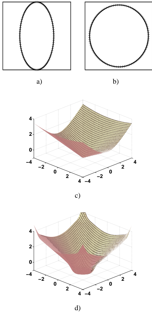
Fig. 2. a) An initial ellipse with half-axes ratio 1:2; c) the same initial condition for the level set approximation; b) the approximate circle computed at the time T = 2.56 by both methods (cross marks correspond to the Lagrangian method); d). the level set function at the time T = 2.56 .
