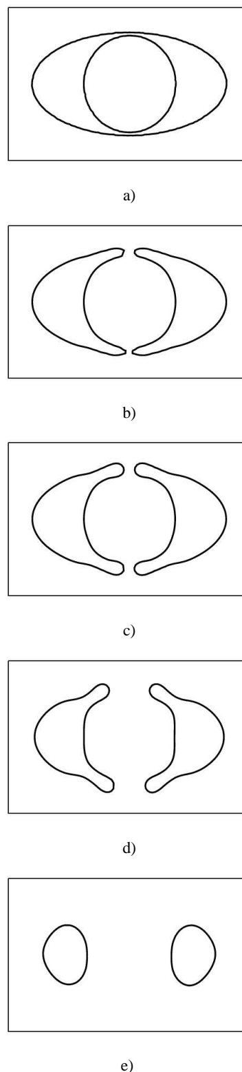
Fig. 7. From top to bottom: Initial condition composed of two curves - a circle within an ellipse a) and its evolution at b): t = 0.00006 ; c): t = 0.0002 ; d): t = 0.002 and e): t = 0.008 .
