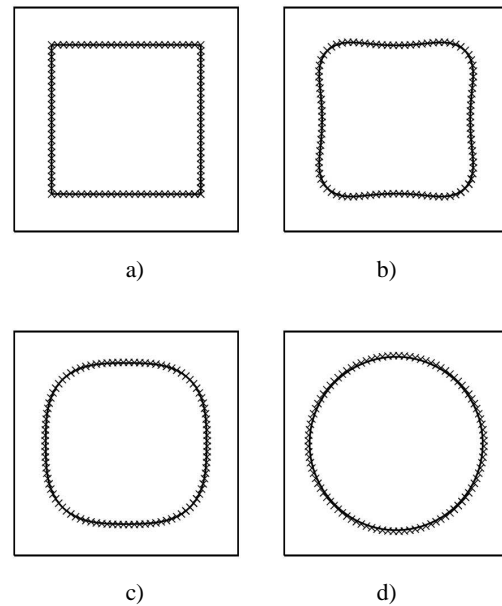
Fig. 4. A square as an initial condition a) and computed evolved curves b): t = 0.001 , c): t = 0.01 and d): t = 0.1 .
