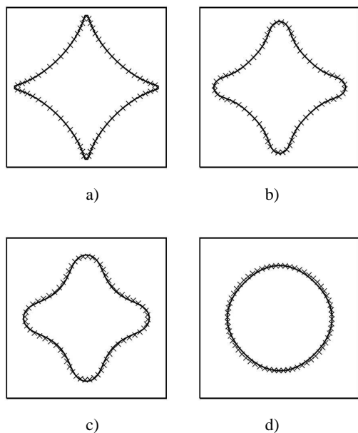
Fig. 6. An asteroide as an initial condition a) and its evolution at b): t = 0.0001 ; c): t = 0.0005 and d): t = 0.005 .
