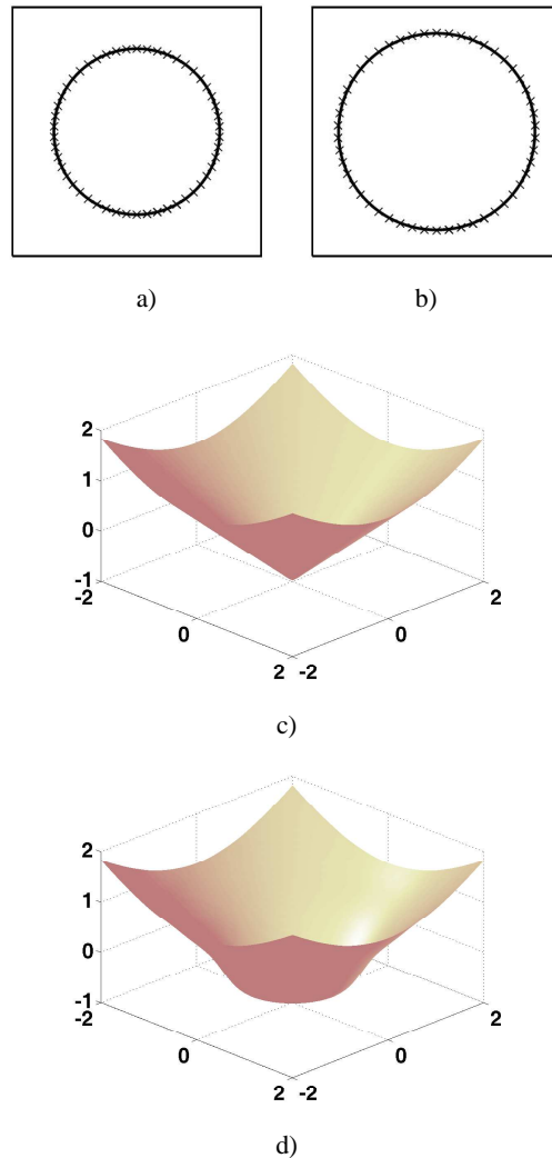
Fig. 1. a) A circle as an initial condition; c) the same initial condition for the level set approximation; b) a circle computed at the time T = 0.5 by both methods (cross marks correspond to the Lagrangian method); d) the level set function at the time T = 0.5 .
